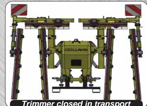
Trimmer closed in transport positioning 8 feet overall width
