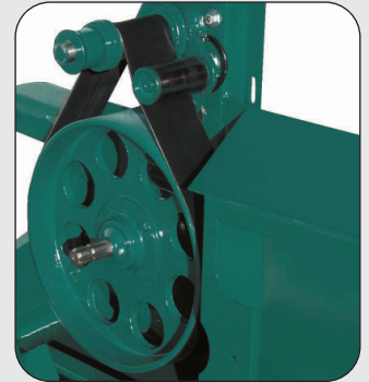
Power band fan speed up system with built-in overrinning clutch
