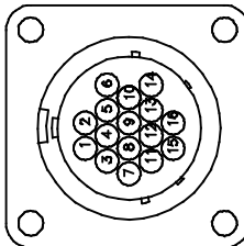
PIN OUT DETAIL
