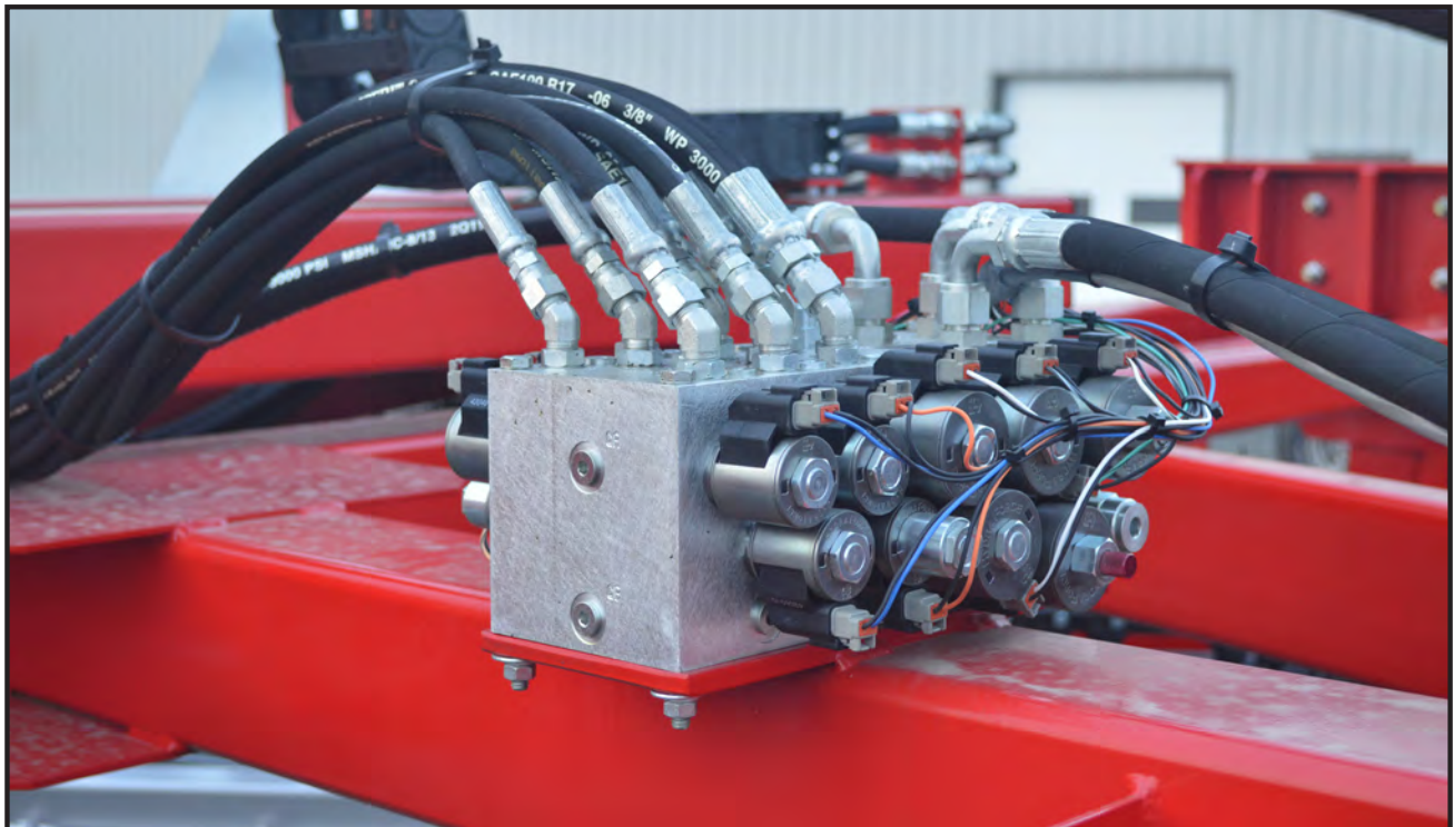
Fig. 8 CONTROL VALVE
