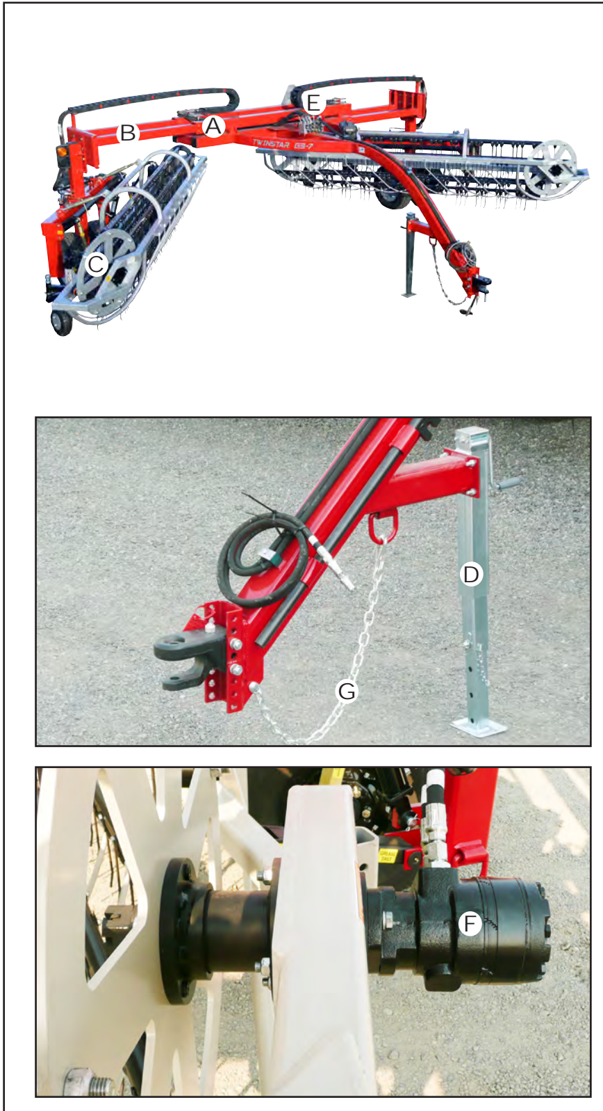
Fig. 1 MACHINE COMPONENTS
