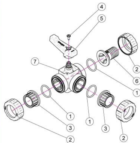
3-WAY VALVE
