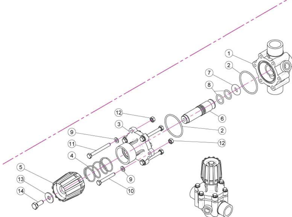
PRESSURE REGULATOR
